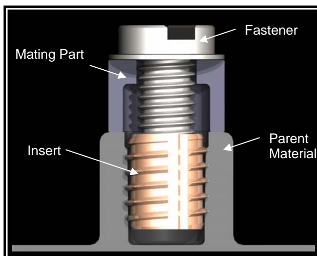
Threaded insert in unsupported assembly.
