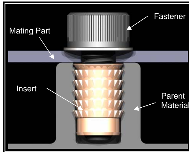
Threaded Insert in a clamped assembly.
